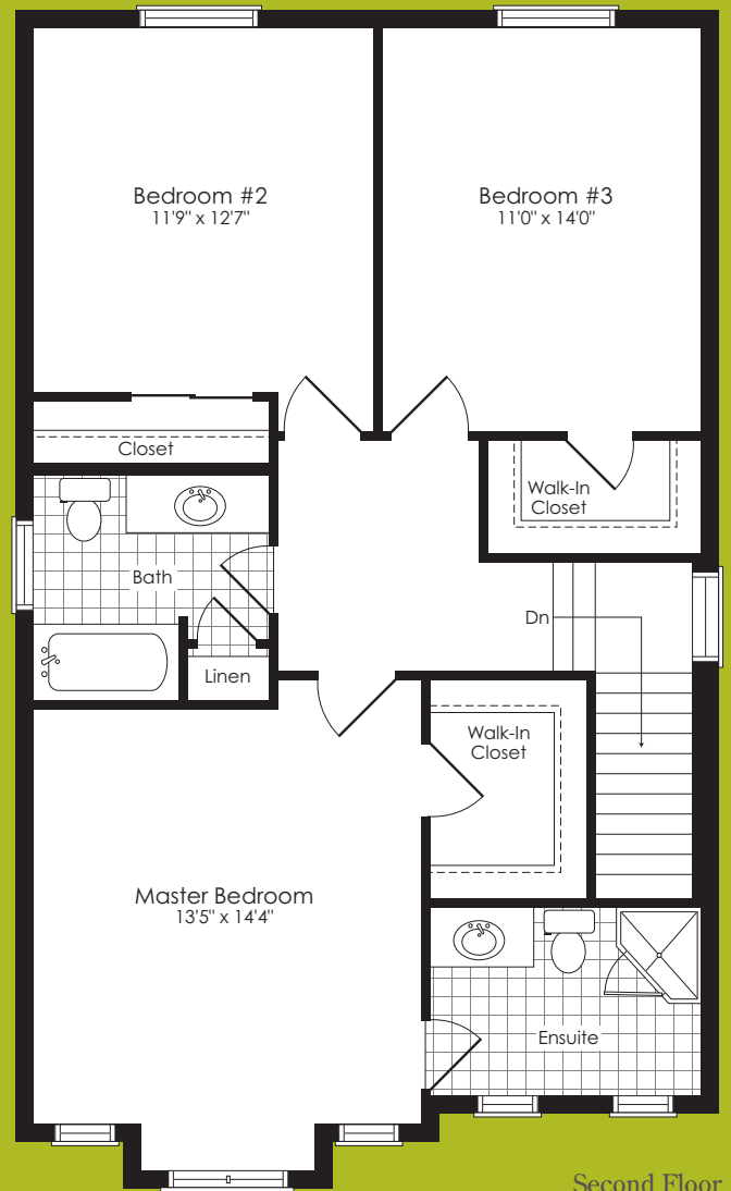
Second Floor
