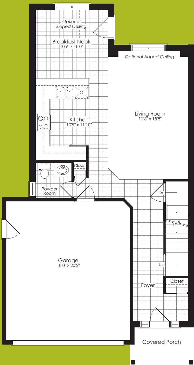
Main Floor
