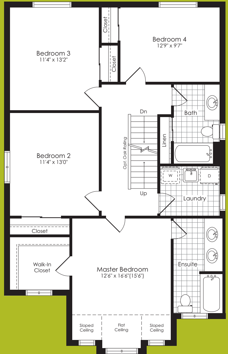
Second Floor
